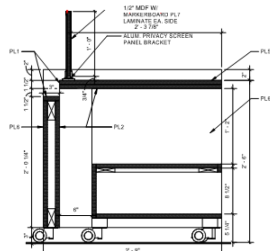
3 INTERIOR CASEWORK SECTION- MEDIA DESK 3/4" = 1'-0"
