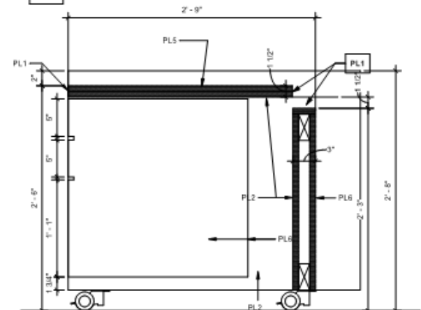
2 CASEWORK - MEDIA DESK KNEE SPACE 3/4" = 1'-0"
